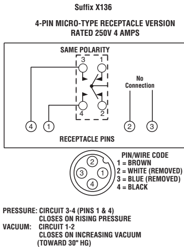
Figure 53 - Without Pilot Light
