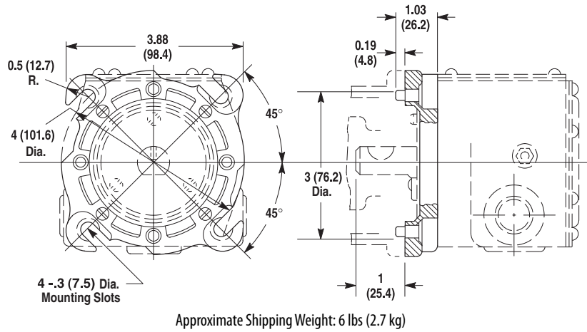
Figure 91 - Flange Mounting (Four-Point) Arrangement Type (Cat. Nos. 808-J3_, -K3_, -M3_, -R3_)
