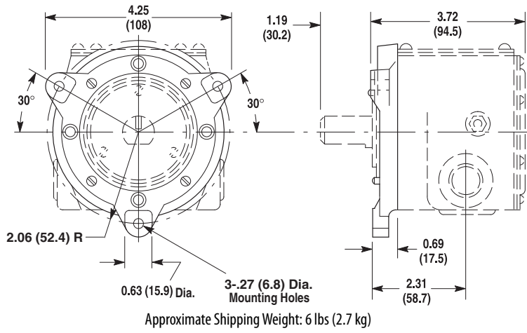
Figure 90 - Flange Mounting (Three-Point) Arrangement Type (Cat. Nos. 808-J2_, -K2_, -M2_, -R2_)
