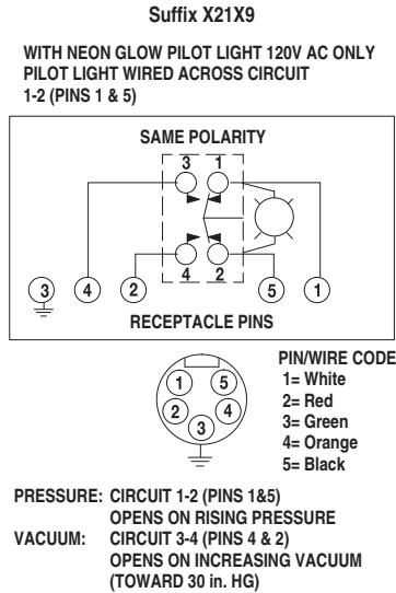
Figure 49 - With Pilot Light (1)
