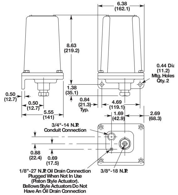
Figure 59 - Type 4 & 13 and 7 & 9 Bellows and Piston Type (1)
