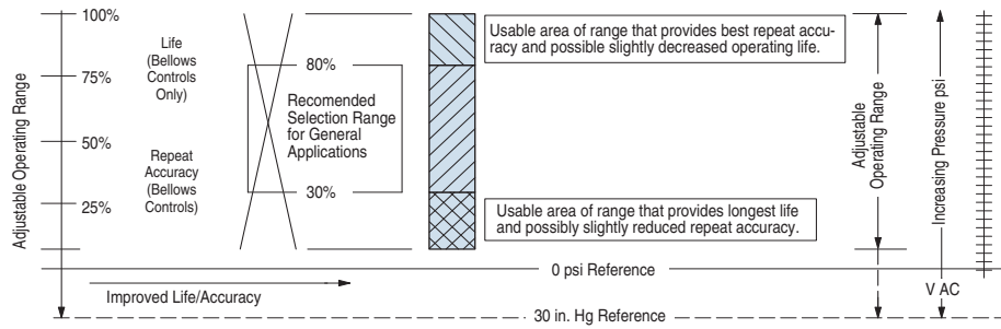
Figure 7 - Repeat Accuracy Versus Mechanical Life
