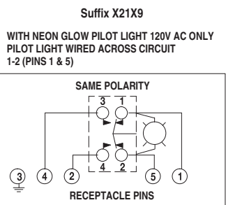
Figure 51 - With Pilot Light (2)
