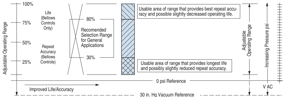
Figure 30 - Repeat Accuracy Versus Mechanical Life
