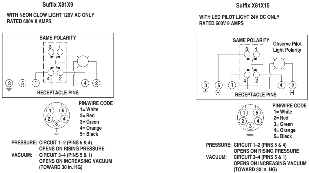
Figure 52 - With Pilot Light
