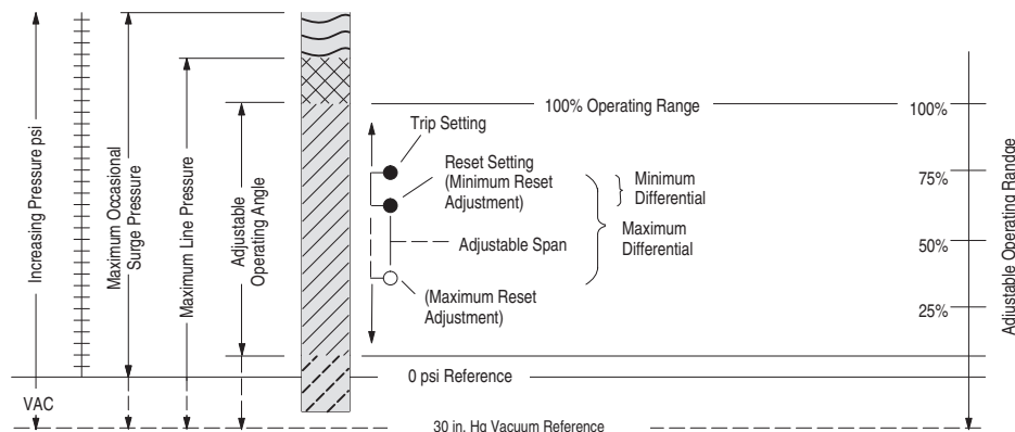
Figure 24 - Graphic to Illustrate Technical Terms
