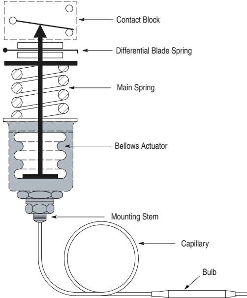
Figure 62 - Basic Mechanical Structure
