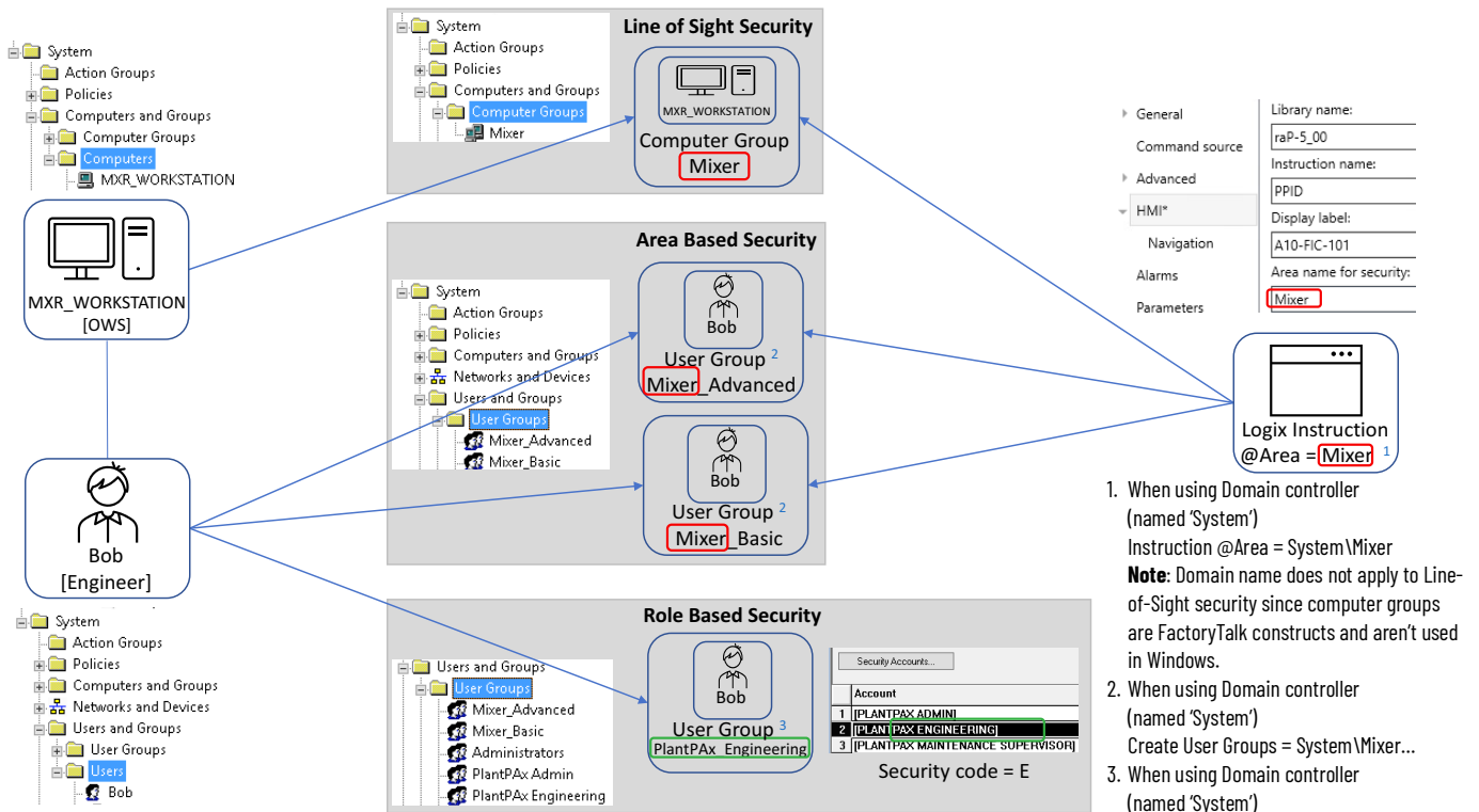
Figure 7 - Security Example with Concurrent Implementation of all Three Security Methods
