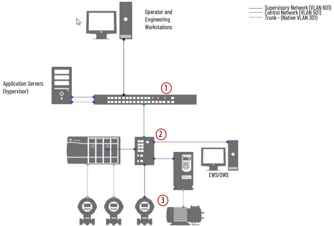
Figure 12 - Simplex - Star Topology Example
