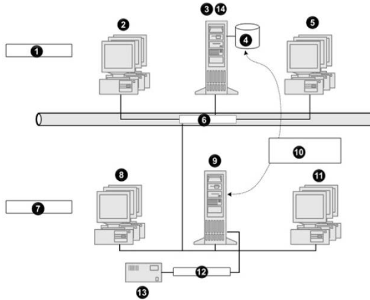
Example FactoryTalk Batch Network
