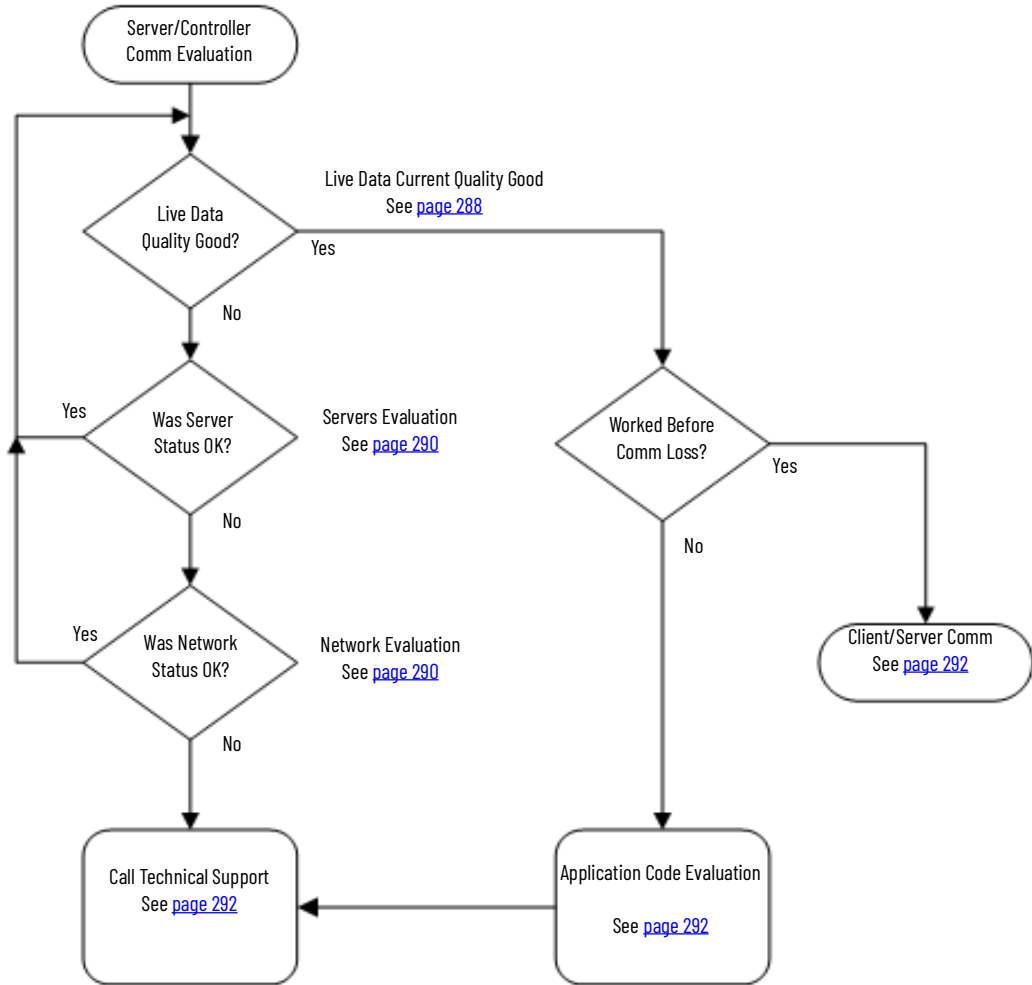
Figure 16 - Resolve Server to Controller Communication
