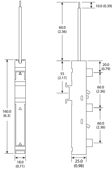
Figure 13 - Cat. No. 141C-18S6L1 1-Pole Adapter
