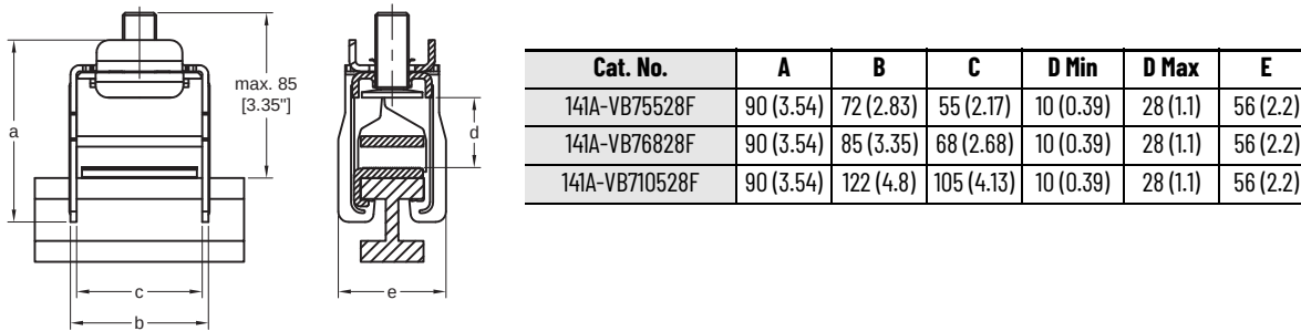
Figure 47 - 141A-BK1 Terminal Cover
