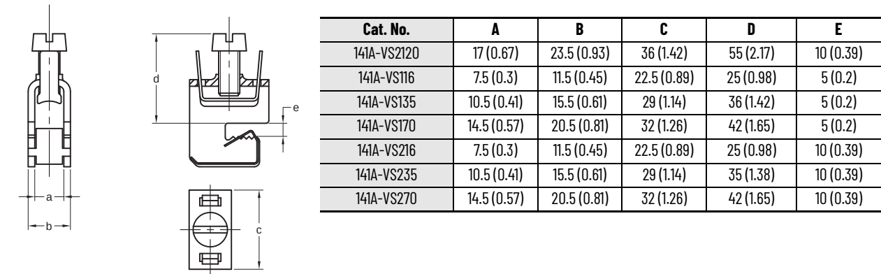
Figure 45 - 141A-VS... Terminals for Connecting to Busbars
