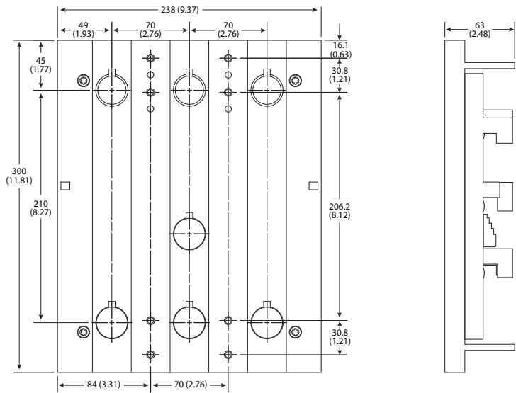
Figure 28 - Cat. No. 141A-W... Panel Mount Adapters
