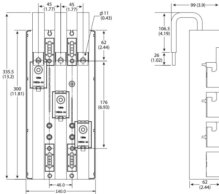
Figure 26 - Cat. No. 141A-GKU
