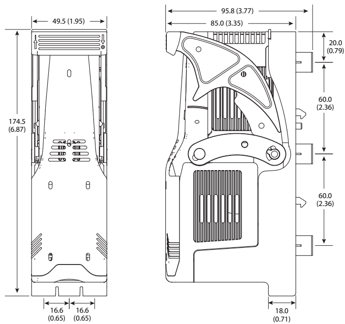
Figure 17 - Cat. No. NFD125 Fuse Switch Disconnecter
