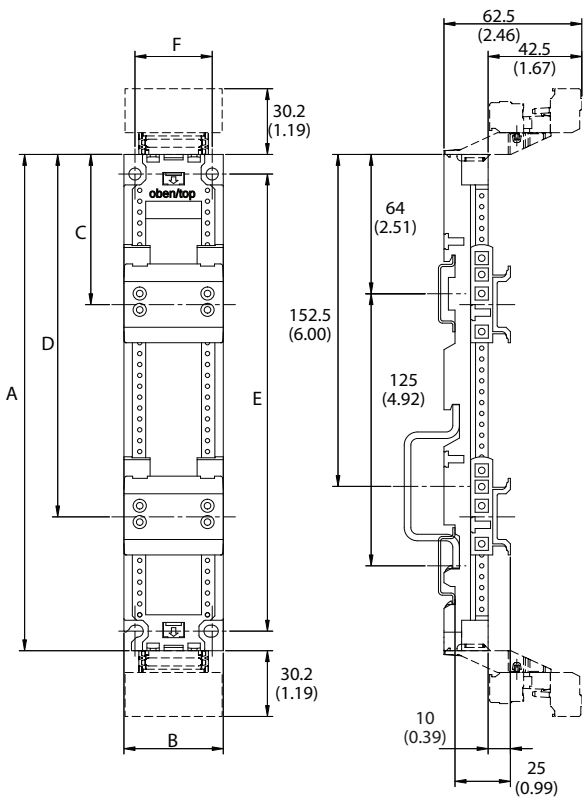
Figure 28 - Cat. No. 141A-W... Panel Mount Adapters
