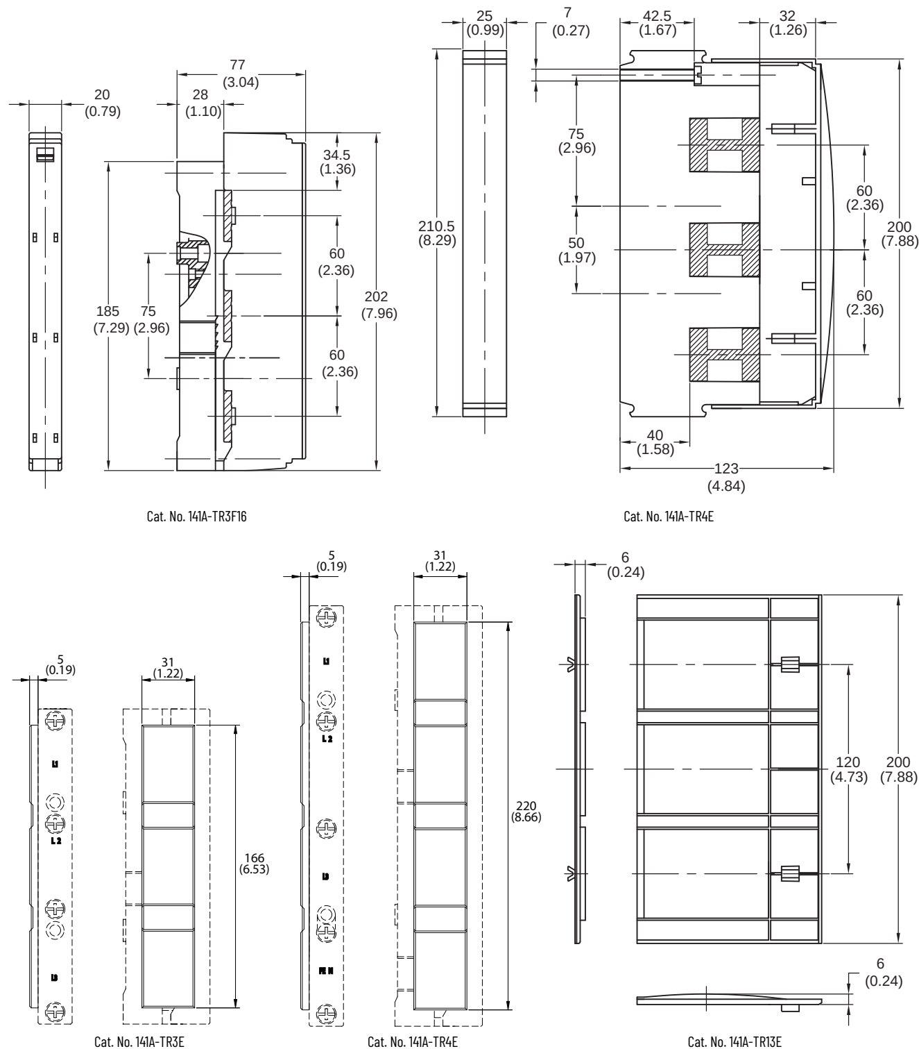
Figure 41 - Cat. Nos. 141A-TR3F16, -T13, -TR3E, -TR4E, and T13E Busbar Supports and End Covers
