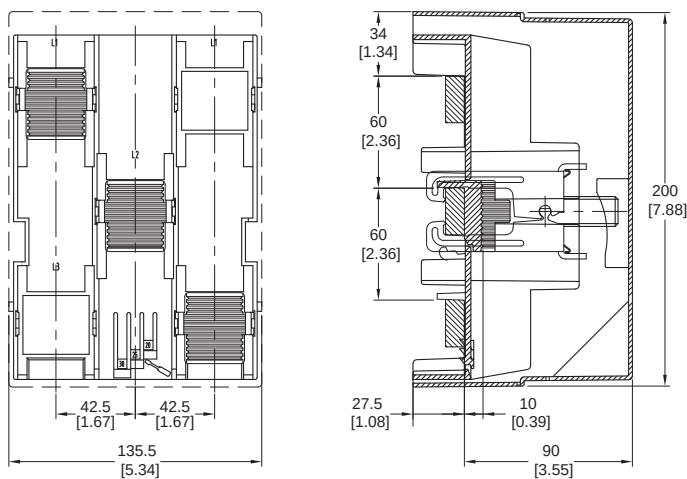
Figure 43 - Cat. Nos. 141A-VN3185, -VN3300R, and -VN3300F
