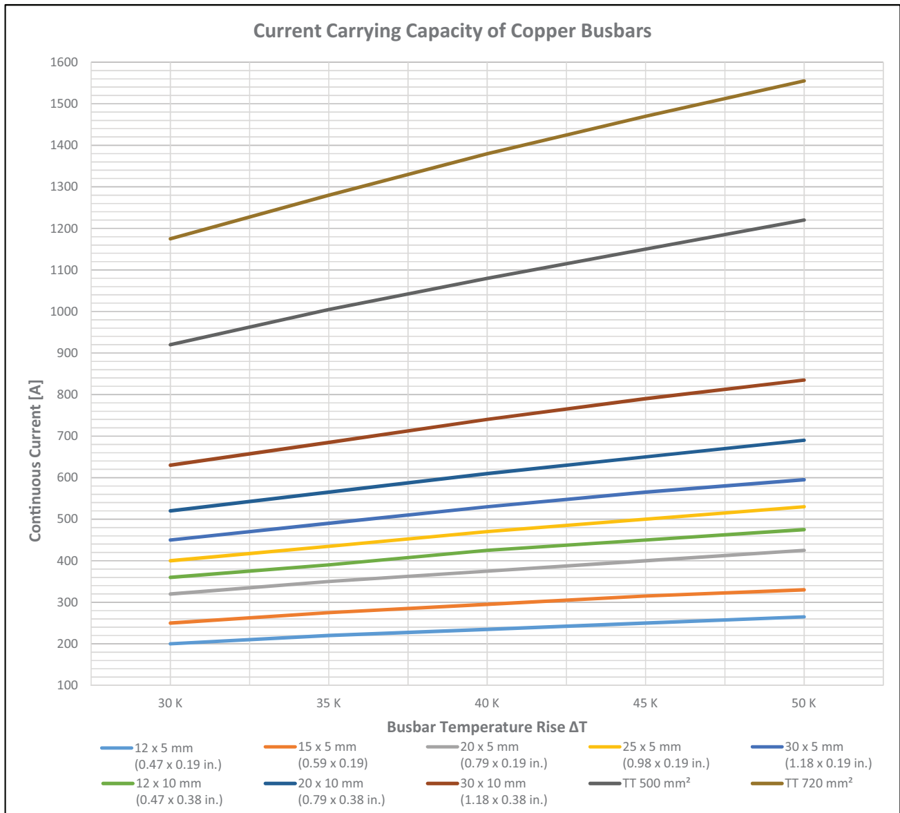
Figure 18 - Current-carrying Capacity of Copper Busbars
