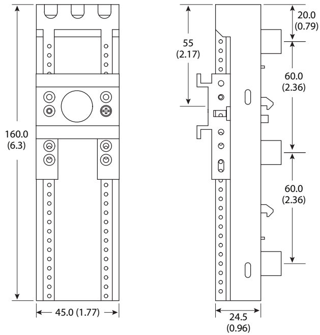
Figure 6 - Cat. No. 141C-45R16 3-Pole Adapter
