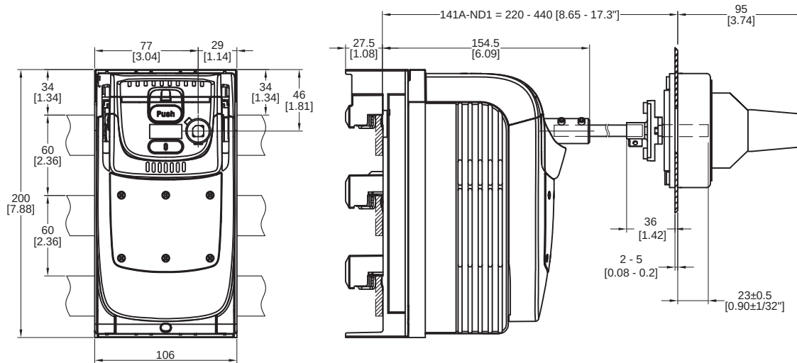
Figure 38 - 141A-N160SB Non-Fused Switch Disconnecter for External Rotary Operating Handle
