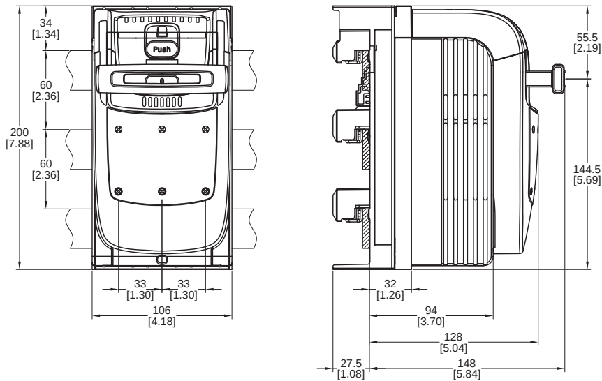
Figure 36 - Cat. No.141A-NFD125SB Fuse Switch Disconnecter for NH Fuses
