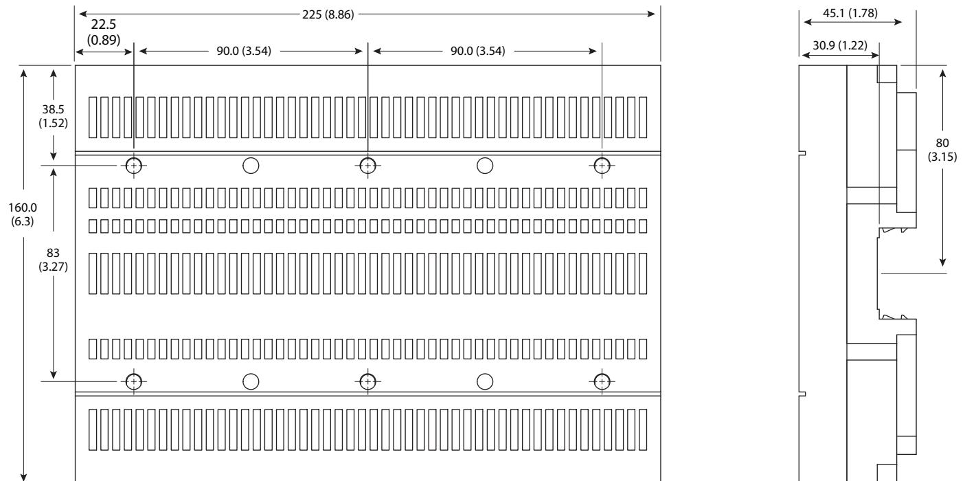
Figure 1 - Cat. No. 141C-B225 Busbar System Base
