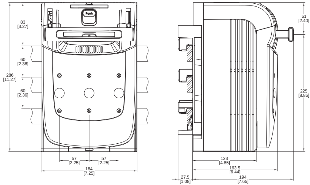
Figure 38 - 141A-N160SB Non-Fused Switch Disconnecter for External Rotary Operating Handle
