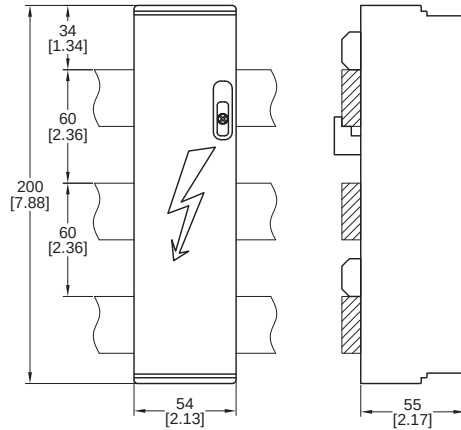
Figure 48 - 141A-BK180, -BK228 Terminal Covers
