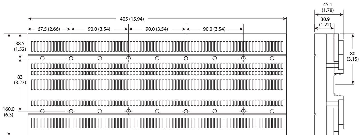
Figure 2 - Cat. No. 141C-B405 Busbar System Base
