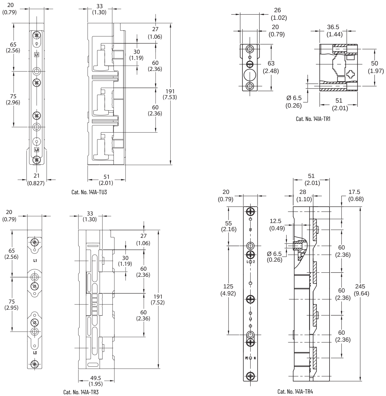
Figure 40 - Cat. Nos. 141A-TU3, -TR1, -TR3, and -TR4 Busbar Supports and End Covers
