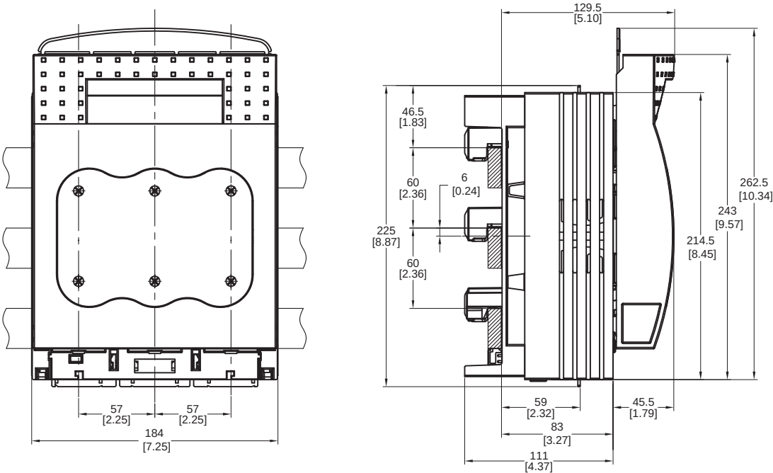
Figure 32 - Cat. No. 141A-NFJ400
