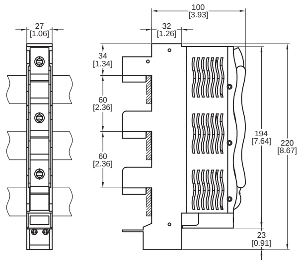
Figure 34 - 141A-NFD160 NH Fuse Switch Disconnecter
