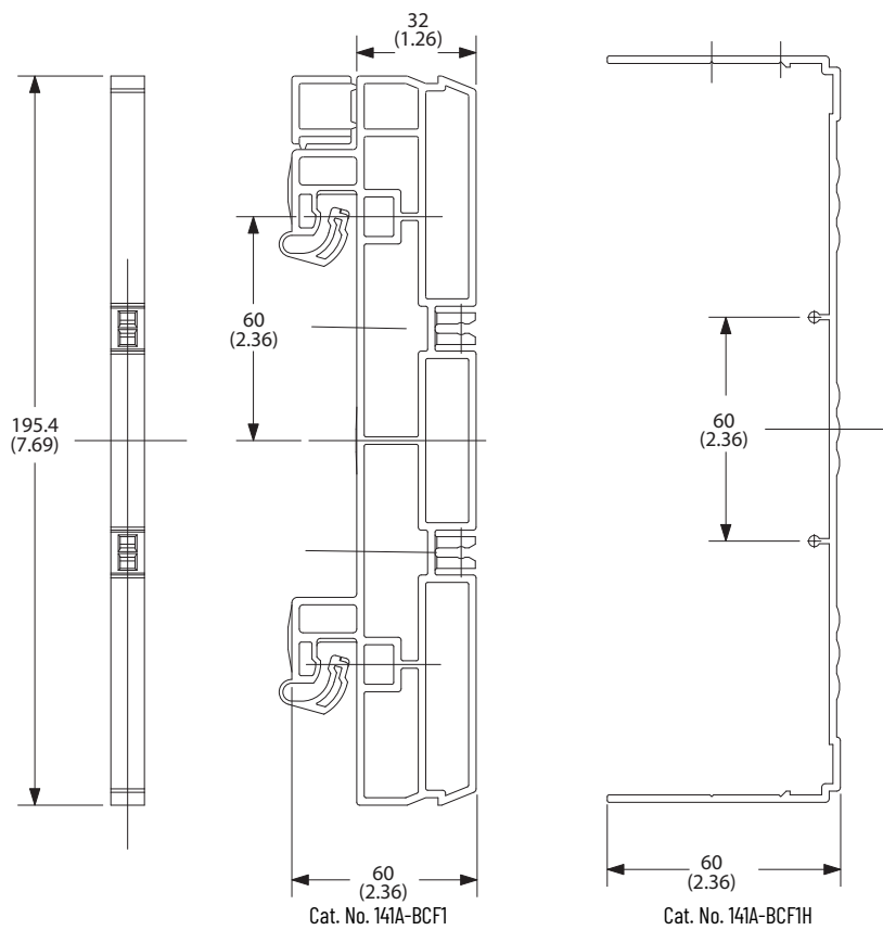
Figure 49 - Cat. Nos. 141A-BCF1, 141A-BCF1H Busbar Cover and Cover Holder
