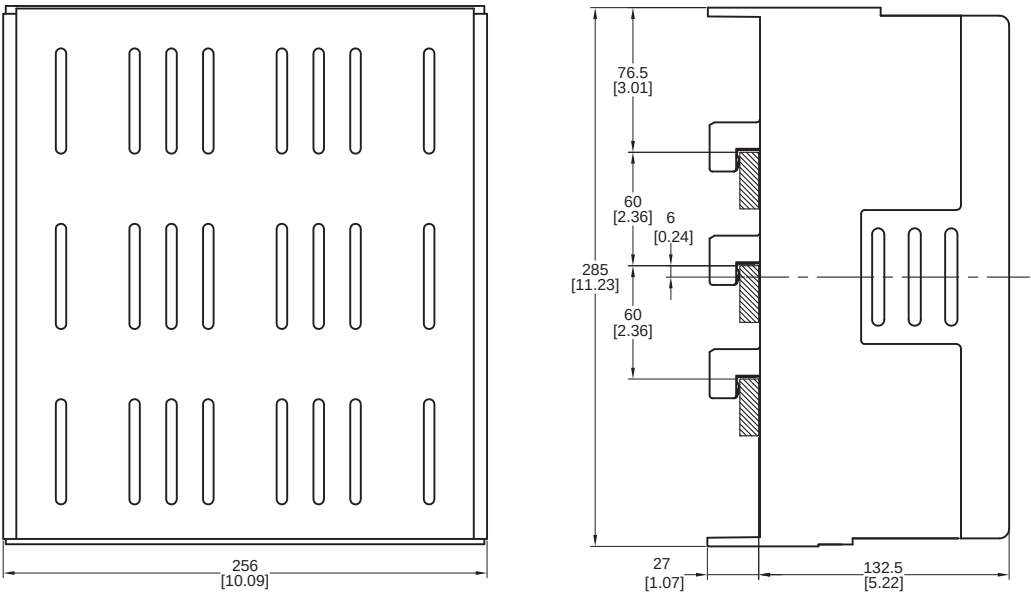
Figure 32 - Cat. No. 141A-NFJ400
