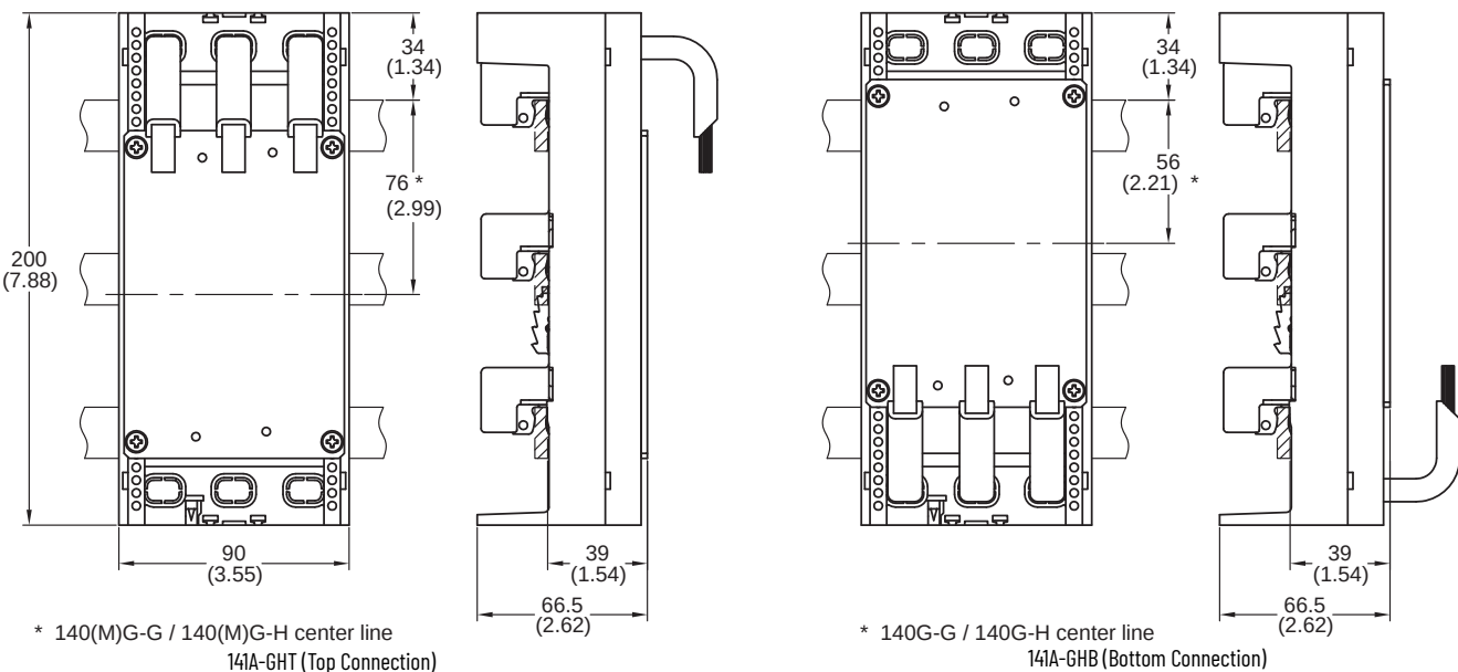
Figure 24 - Cat. Nos. 141A-GHT, -GHB
