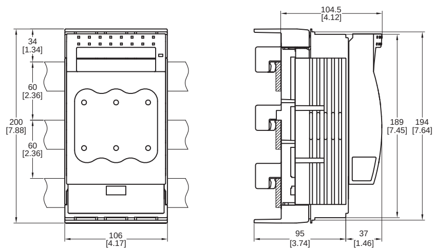
Figure 30 - Cat. Nos. 141A-NFJ30C, -60C, and -100C
