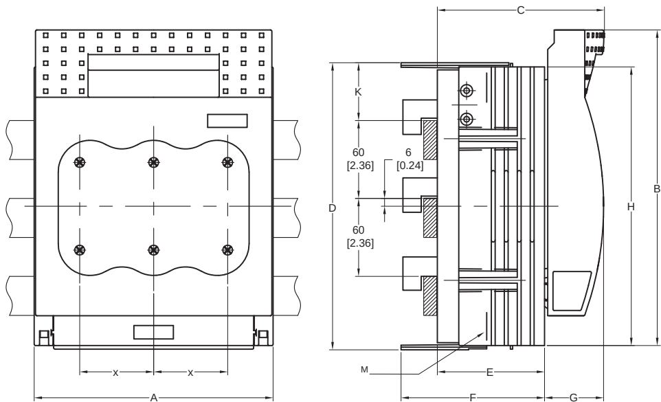
Figure 35 - 141A-NFD... NH Fuse Switch Disconnecter
