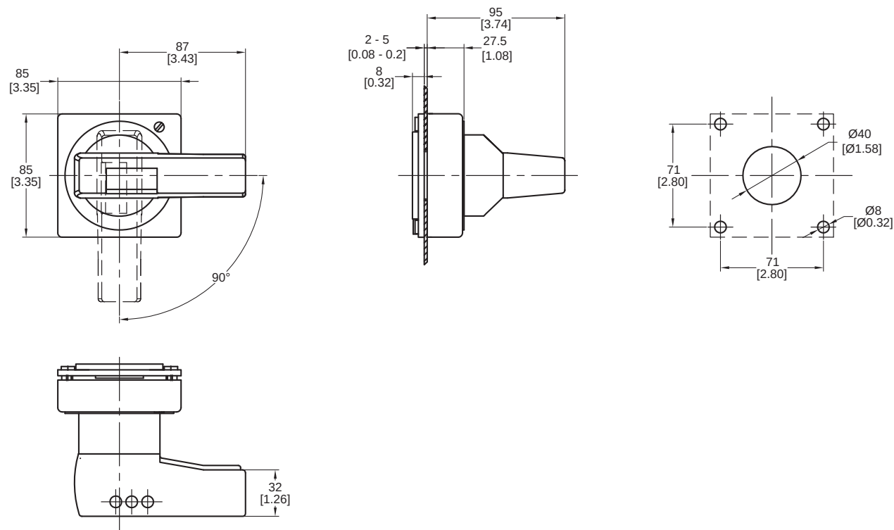
Figure 39 - 141A-NDRY66 Operating Handles
