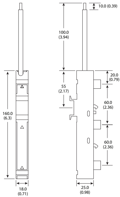
Figure 17 - Cat. No. NFD125 Fuse Switch Disconnecter
