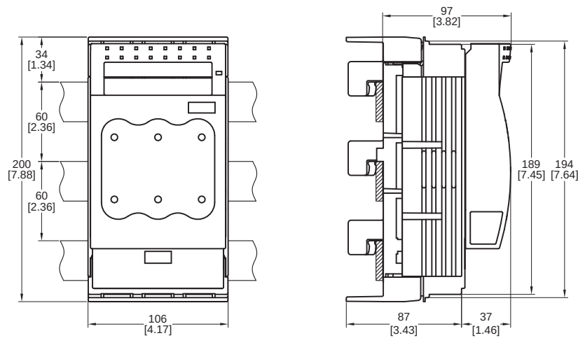
Figure 34 - 141A-NFD160 NH Fuse Switch Disconnecter
