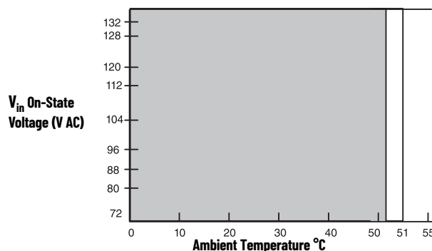
Figure 8 - 1794-0A16, 1794-0A16K Derating Curve
