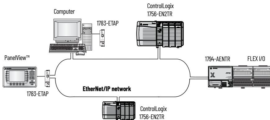
Figure 2 - FLEX I/O in a DLR Topology
