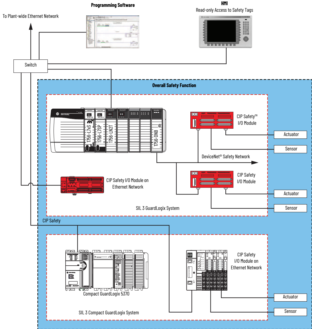
Figure 1 - Typical SIL Function
