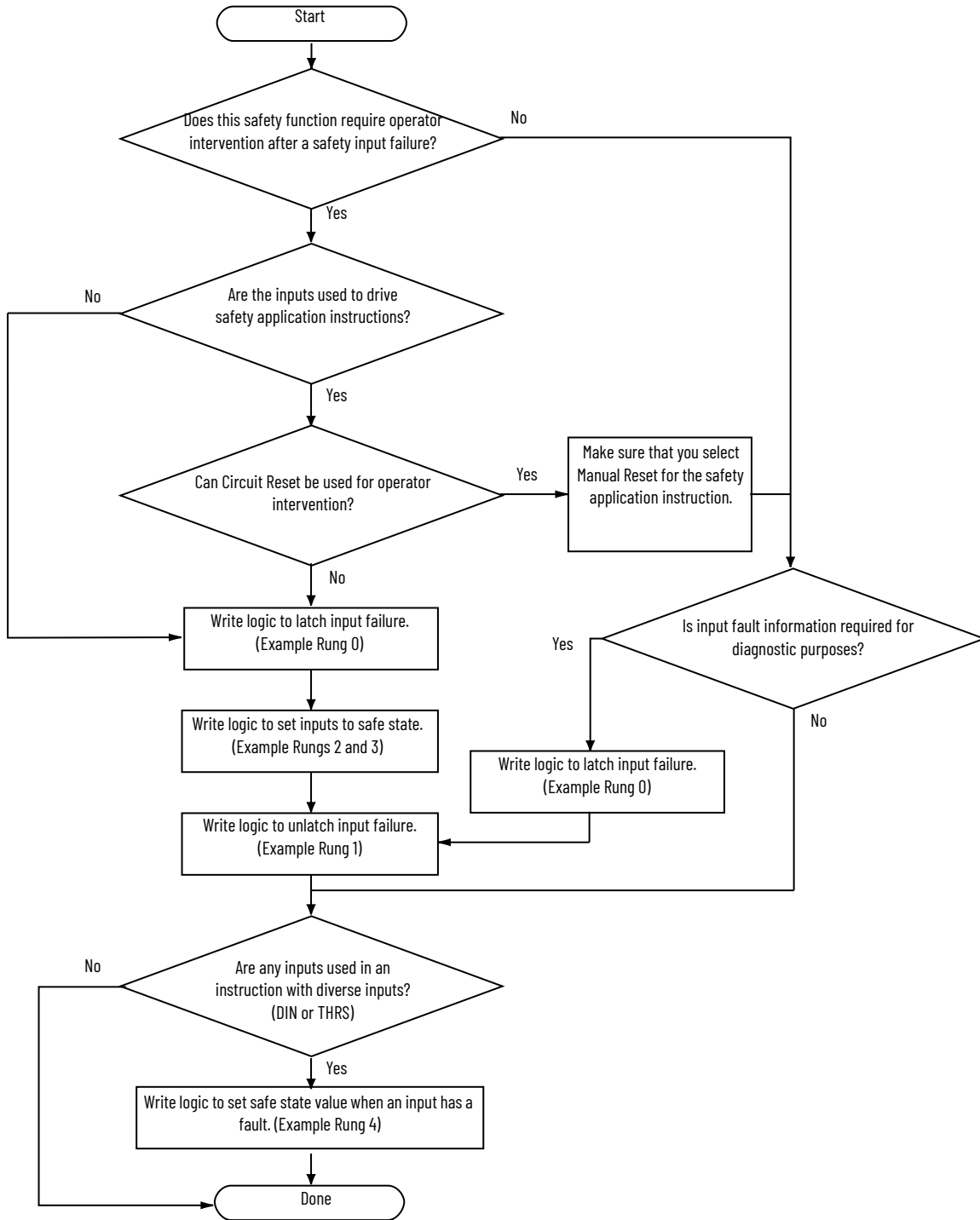
Figure 22 - Input Fault Latch and Reset Flowchart
