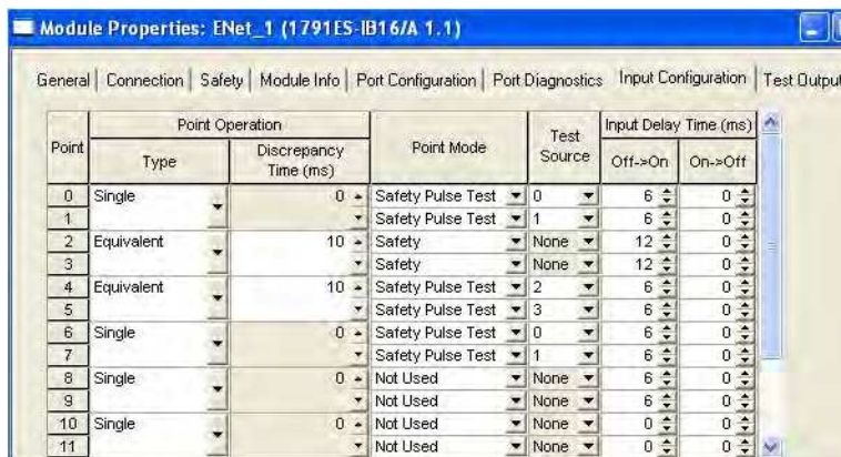
Figure 13 - Input Configuration
