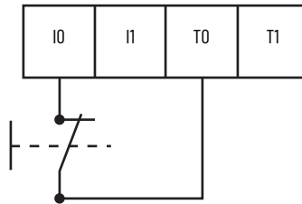
Figure 11 - Input Wiring
