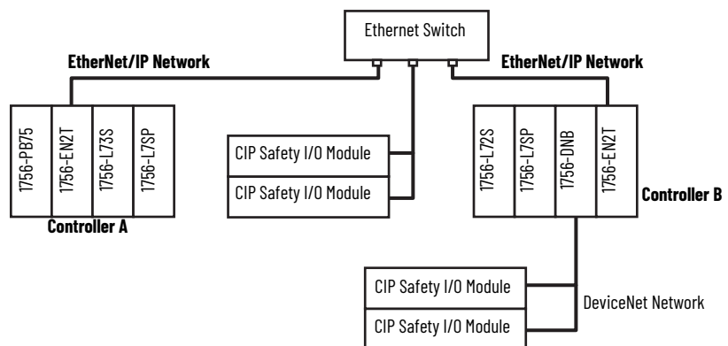
Figure 4 - Peer-to-peer Communication via EtherNet/IP Bridges and the EtherNet/IP Network
