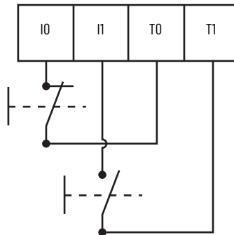
Figure 12 - Input Wiring in Pairs
