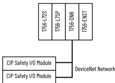
Figure 5 - Communication via a DeviceNet Bridge
