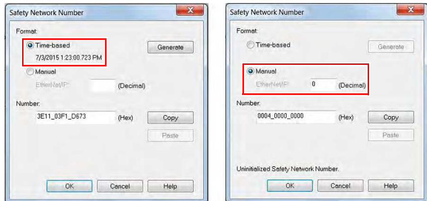
Figure 10 - SNN Formats
