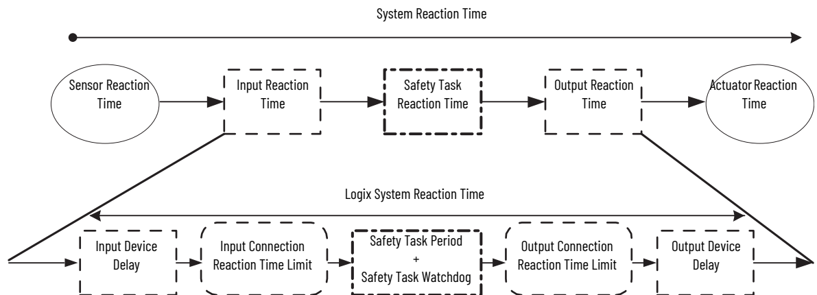
Figure 19 - System Reaction Time
