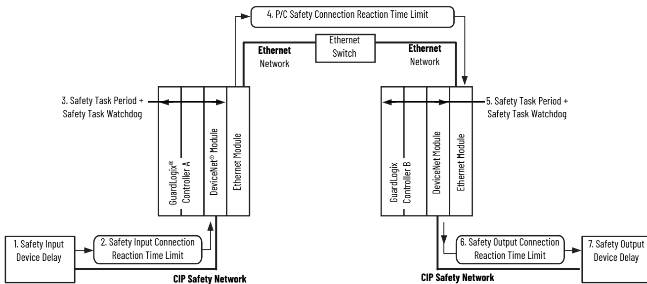
Figure 21 - Logix System Reaction Time for Input to Controller A Logic to Controller B Logic to Output Chain
