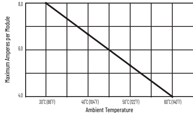
1769-0A16 Maximum Amperes per Module Versus Temperature
