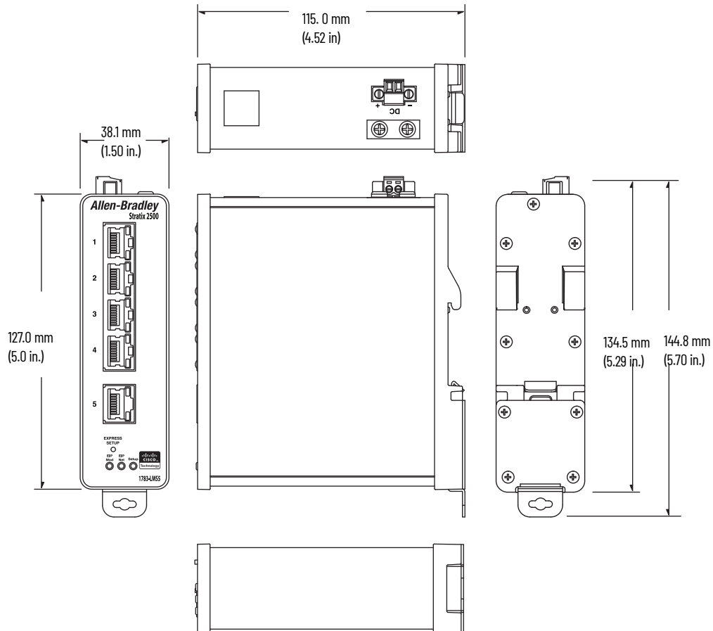
Figure 13 - 1783-LMS5 Switch Dimensions
