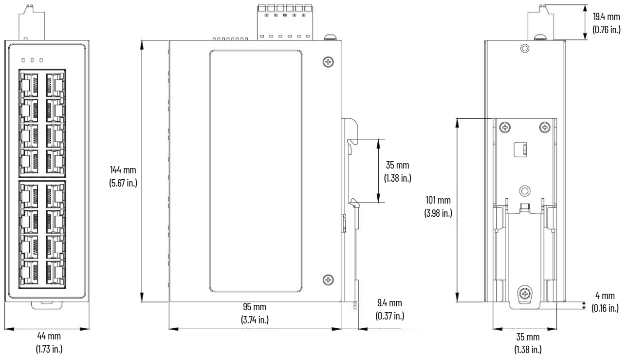
Figure 12 - Stratix 2100 16 Port Switch Dimensions (1783-USP16T, 1783-USP16TG, 1783-USP16TGK)
