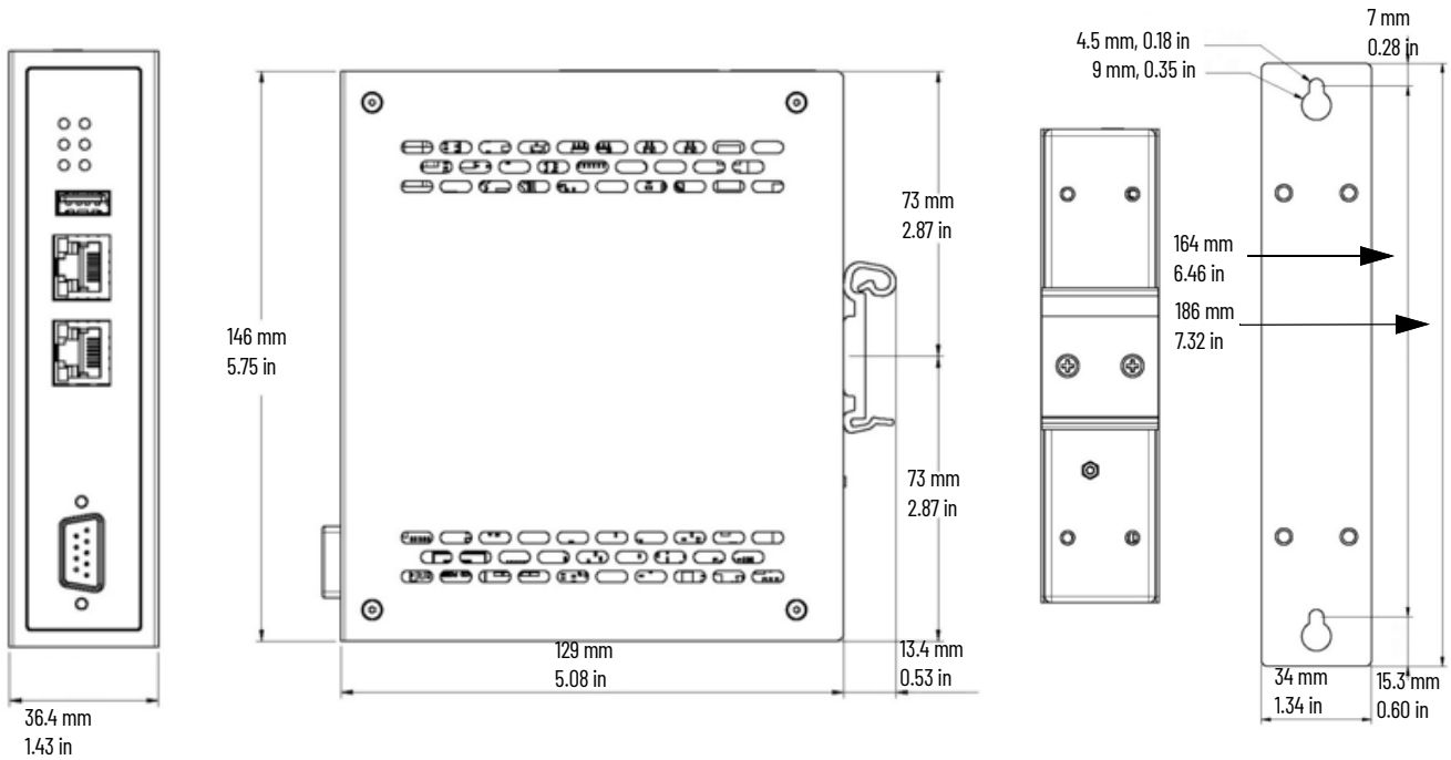
Figure 16 - Stratix 4300 Remote Access Router - 1783-RA5TGB, 1783-RA5TGW, 1783-RA5TGC4G, 1783-RA5TGC4G
