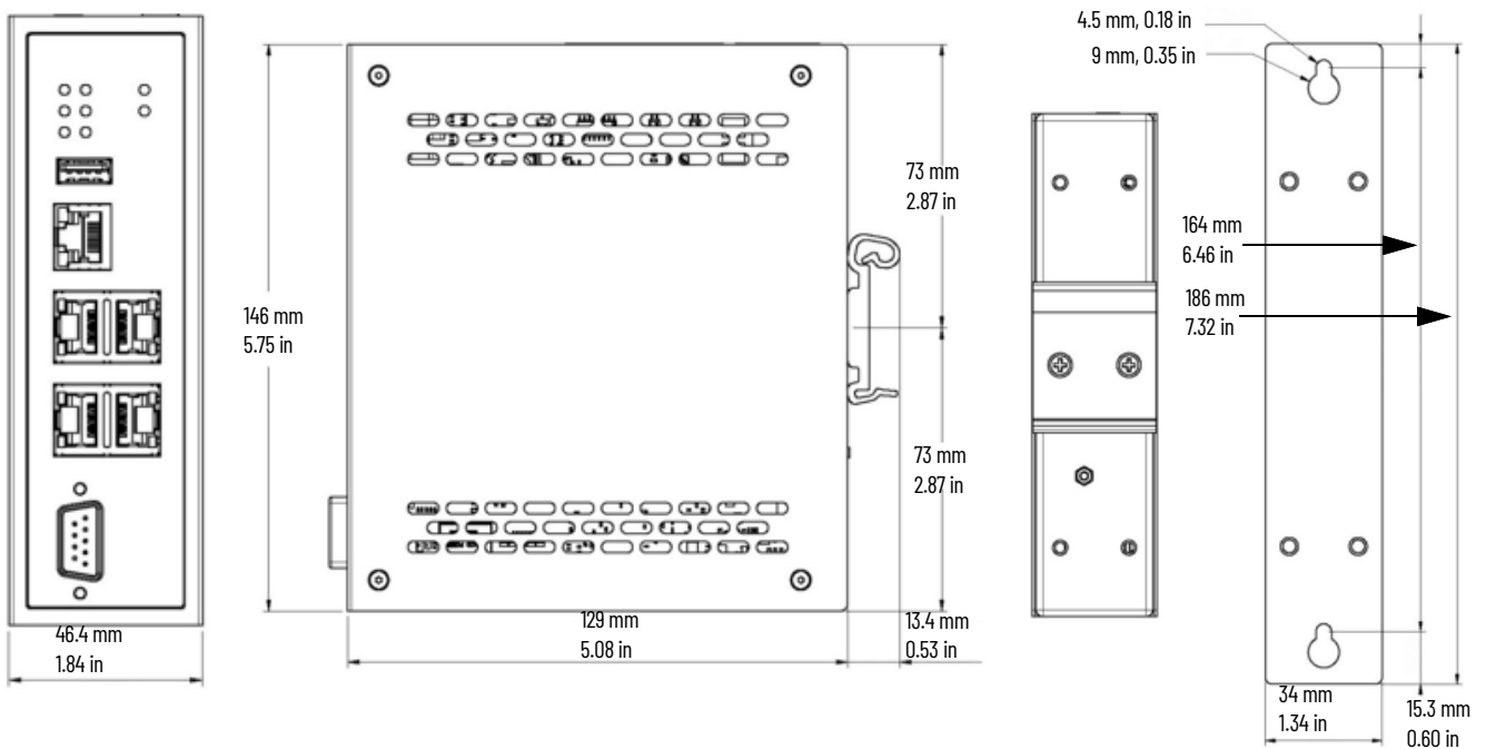
Figure 16 - Stratix 4300 Remote Access Router - 1783-RA5TGB, 1783-RA5TGW, 1783-RA5TGC4G, 1783-RA5TGC4G
