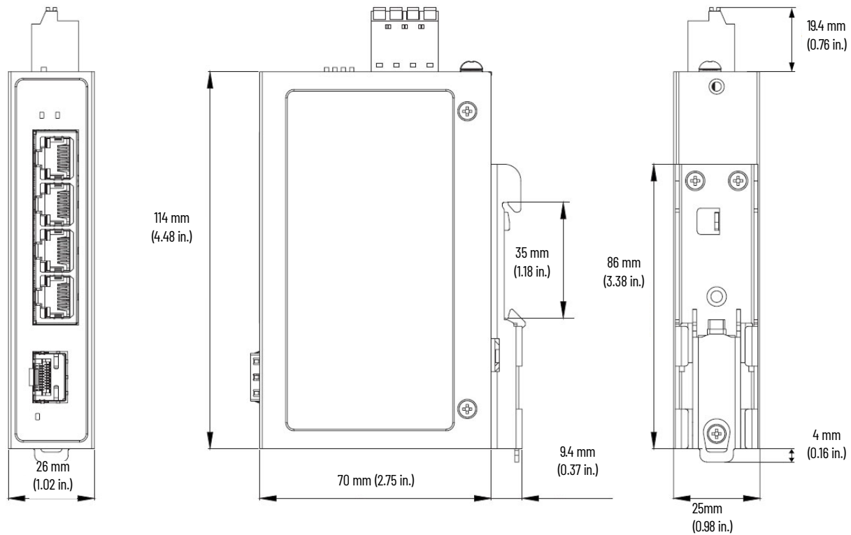
Figure 10 - Stratix 2100 5 Port Switch Dimensions (1783-USP5T, 1783-USP5TG, 1783-USP5TGK, 1783-USP1S4T, 1783-USP1S4TG, 1783-USP1T64TGE)
