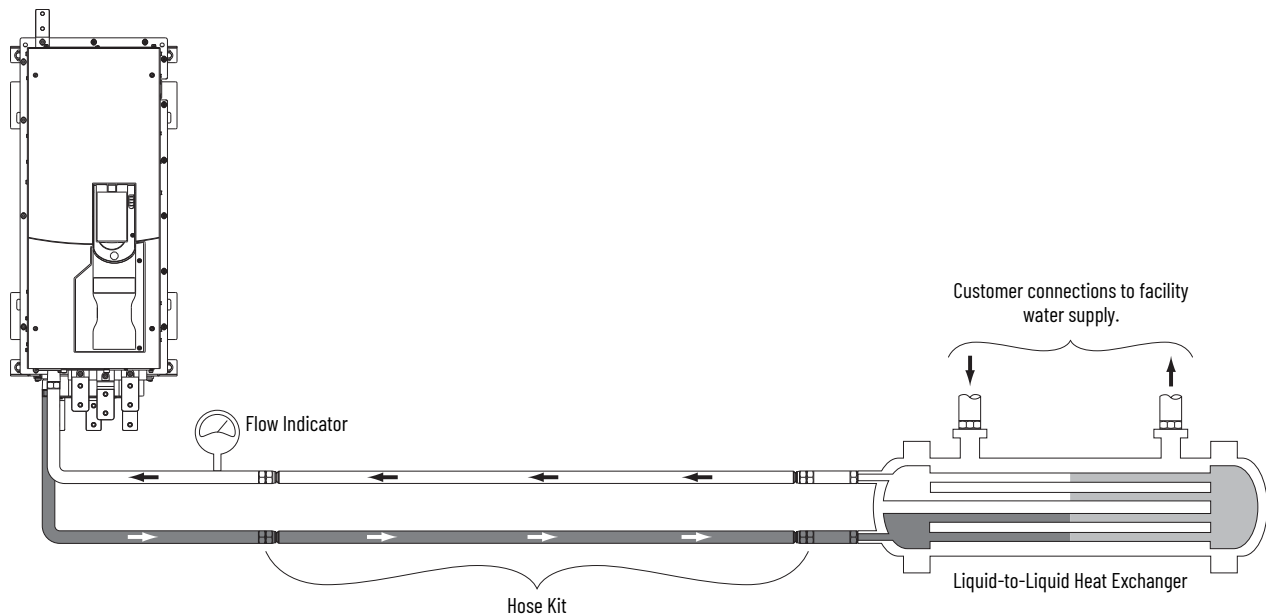
PowerFlex 755TR Liquid-cooled Drive (Frame 6L Shown)
