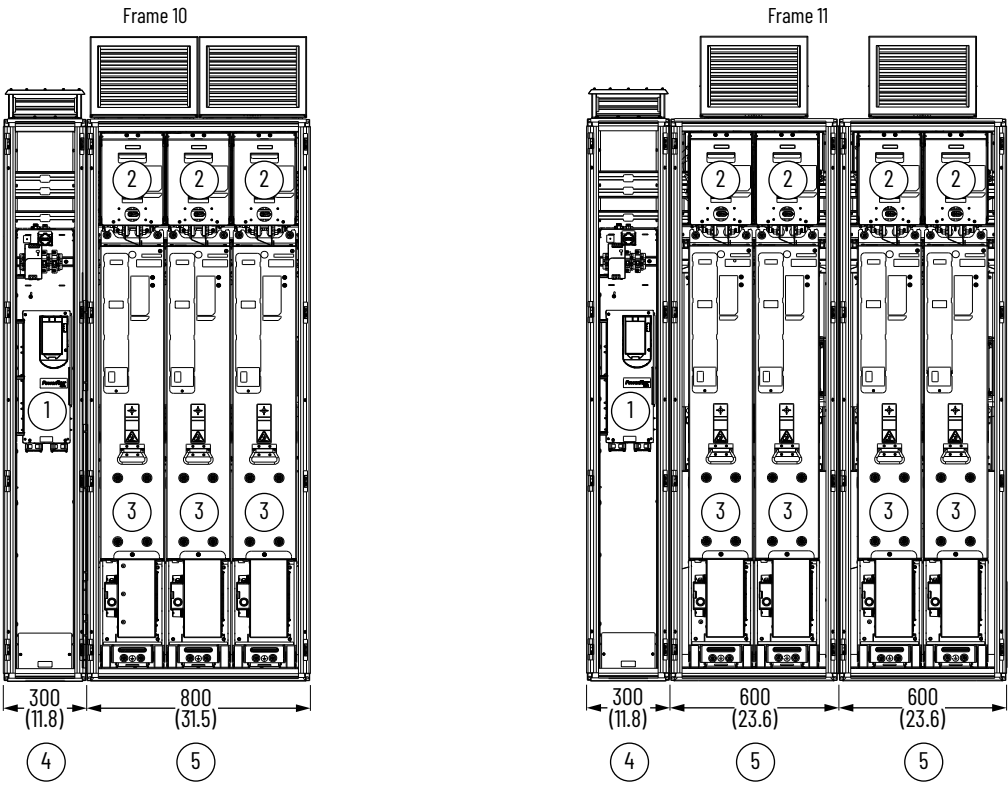
All cabinet enclosures are 600 mm (23.6 in.) deep. IP54, UL Type 12 Enclosure Shown.
