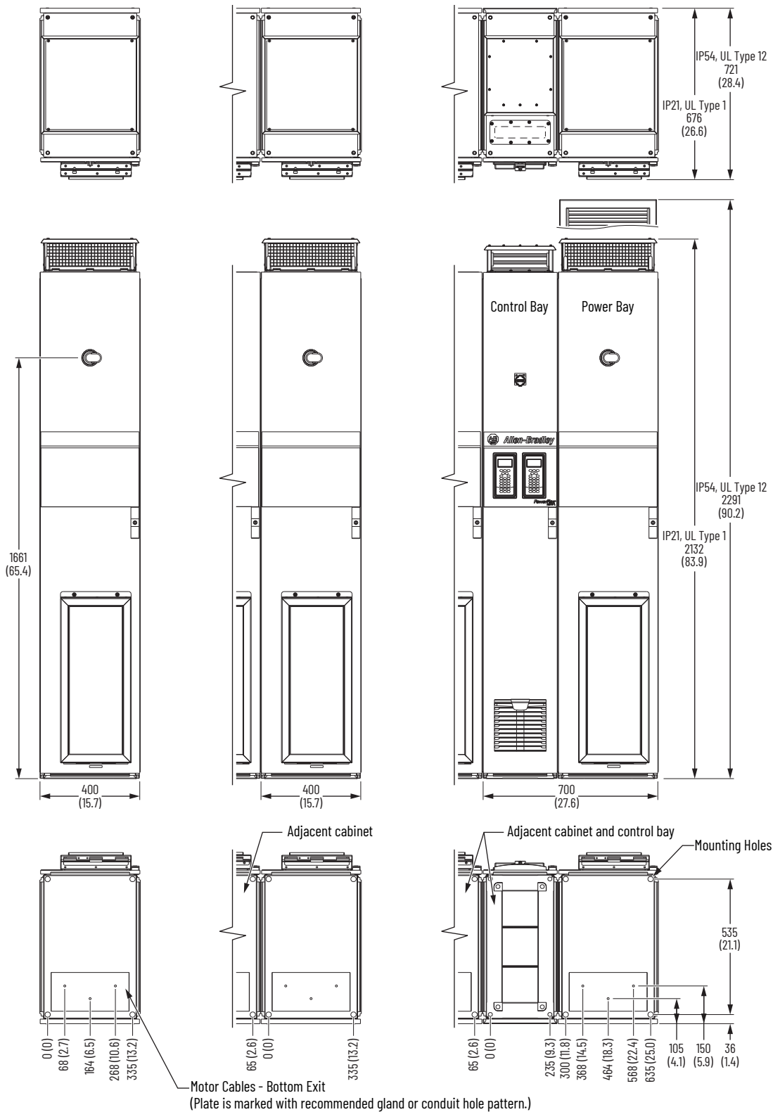
Frame 8 Common Bus Inverters Top, Front, and Bottom Views
