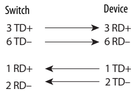
Figure 6 - Four Twisted-pair Straight-through Cable Schematics
