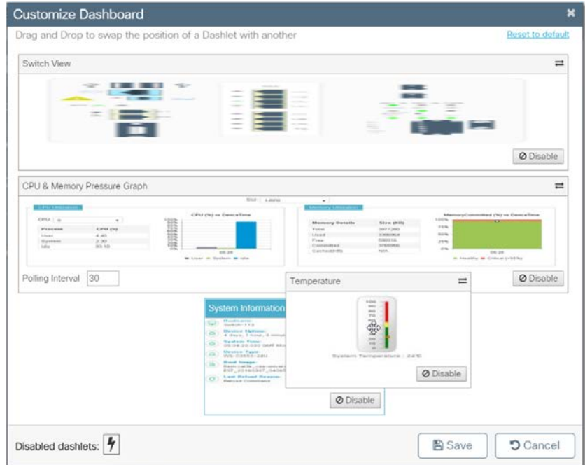
Figure 19 - Customize Dashboard
