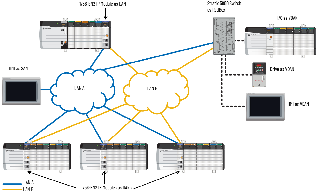
Figure 30 - PRP Topology with Stratix 5800 Switch as RedBox
