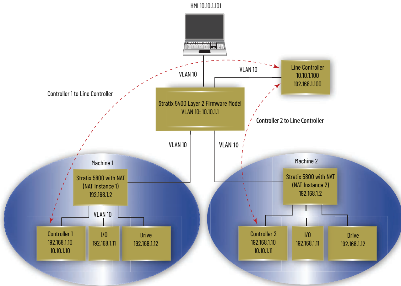
Figure 29 - Layer 2 Example with NAT in Stratix 5800 Switch
