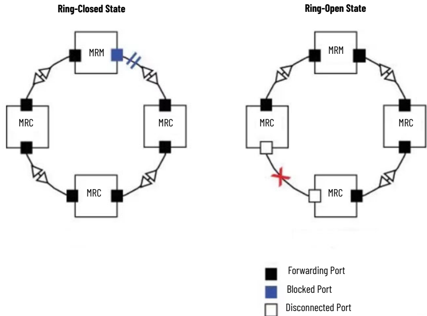
Figure 27 - MRP Ring States
