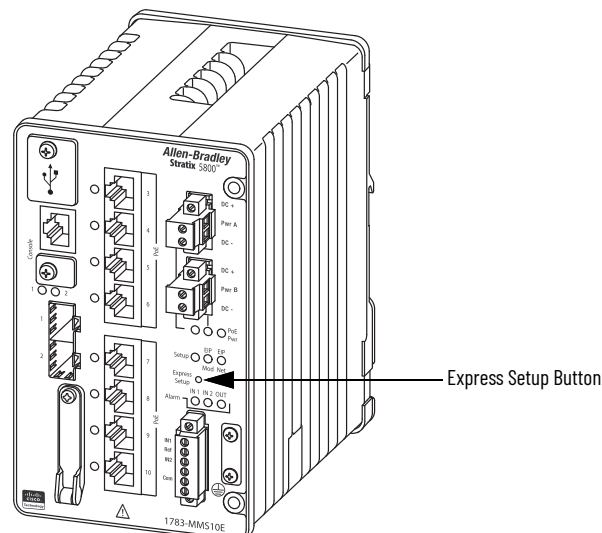
Figure 12 - Stratix 5800 Switch
