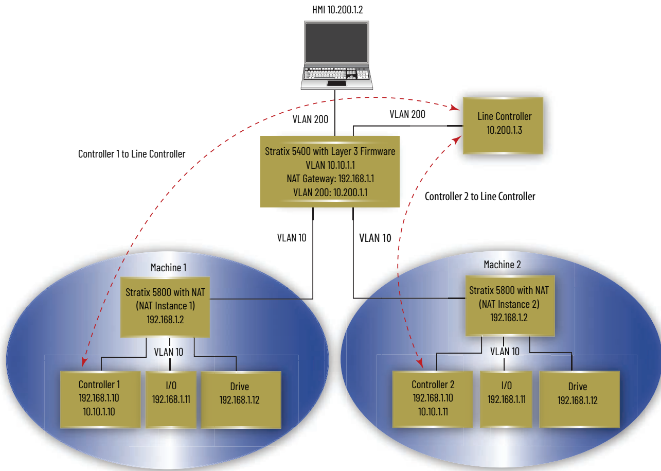
Figure 28 - Layer 3 Example with NAT in Stratix 5800 Switch
