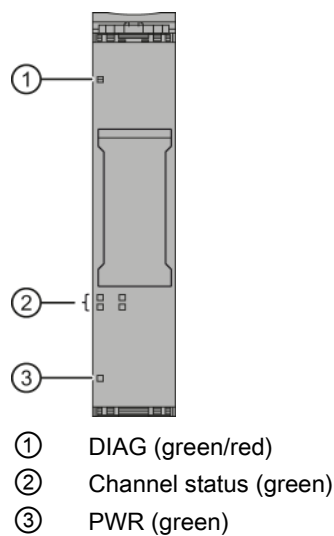
Figure 5-1 LED display
