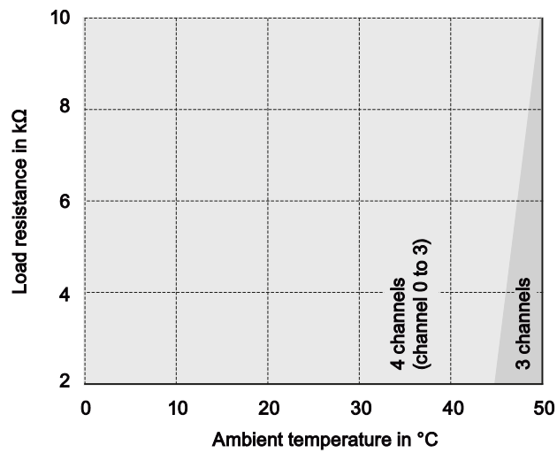
Figure 6-4 Derating trend voltage output (vertical)
