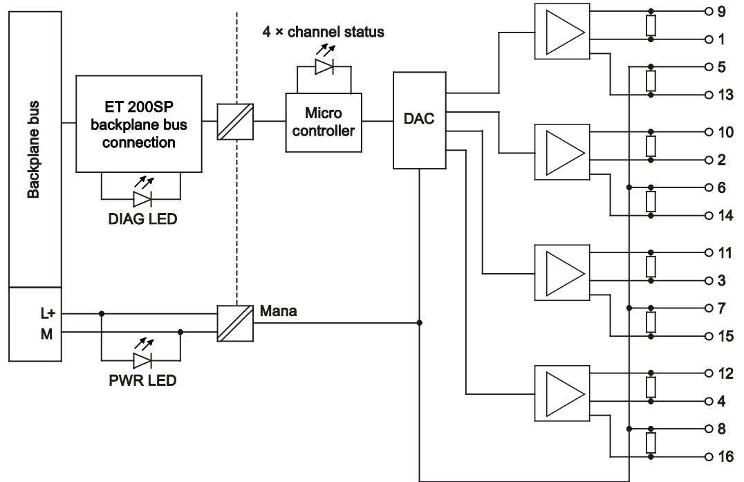
Figure 3-1 Schematic circuit diagram for AQ 4xUI ST
