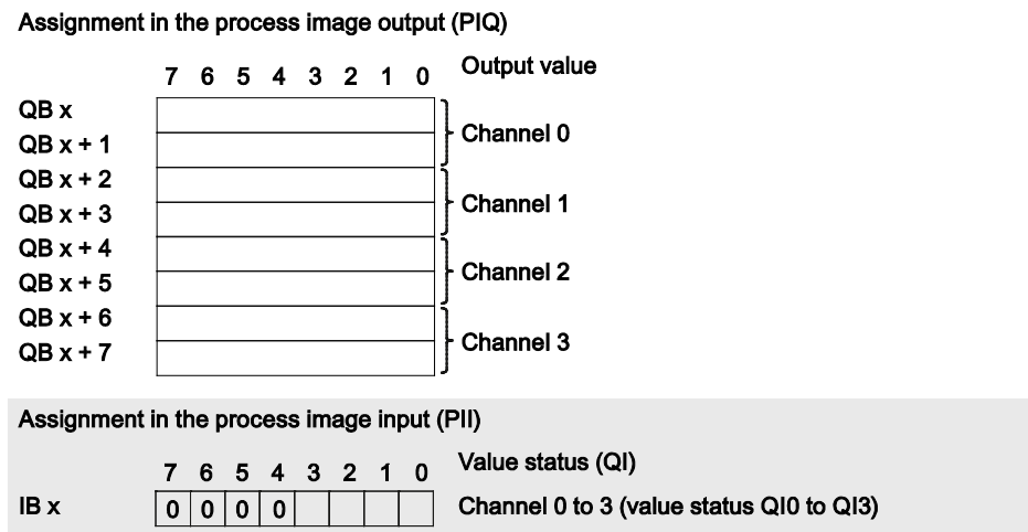
Figure 4-1 Address space of the AQ 4xU/I ST with value status
