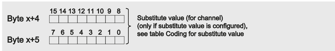
Figure A-3 Structure byte x up to x+5 for the channel 0 to 3
